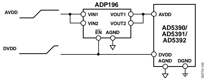
Figure 43. AV_{DD} Power Supply Controlled by a Load Switch
