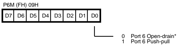
Figure 51. Port 6 Mode Register (F 09: Write Only)
