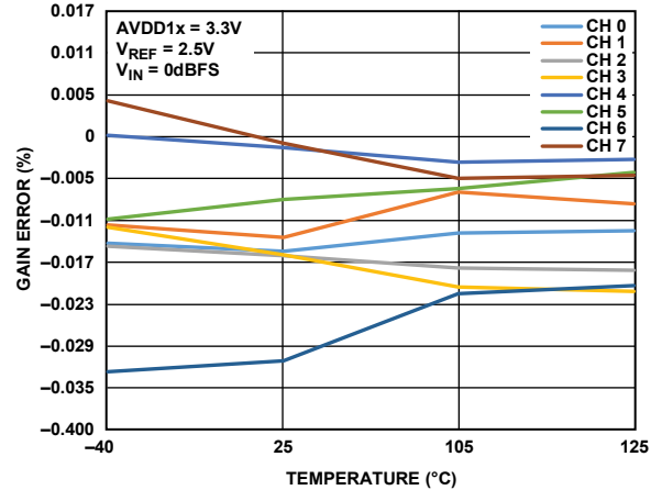
Figure 53. Gain Error vs. Temperature, Low Power Mode
