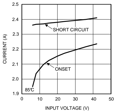
Figure 31. Current Limit 3.3 V OUT at 85°C
