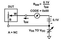
Figure 37. Incremental On Resistance
