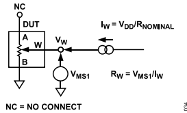
Figure 35. Wiper Resistance
