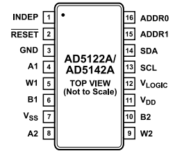
Figure 5. 16-Lead TSSOP Pin Configuration
