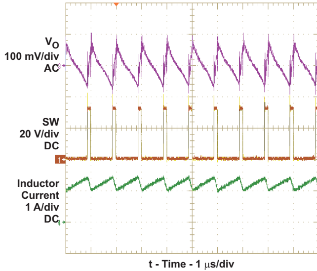
Figure 11. Switching Waveform
