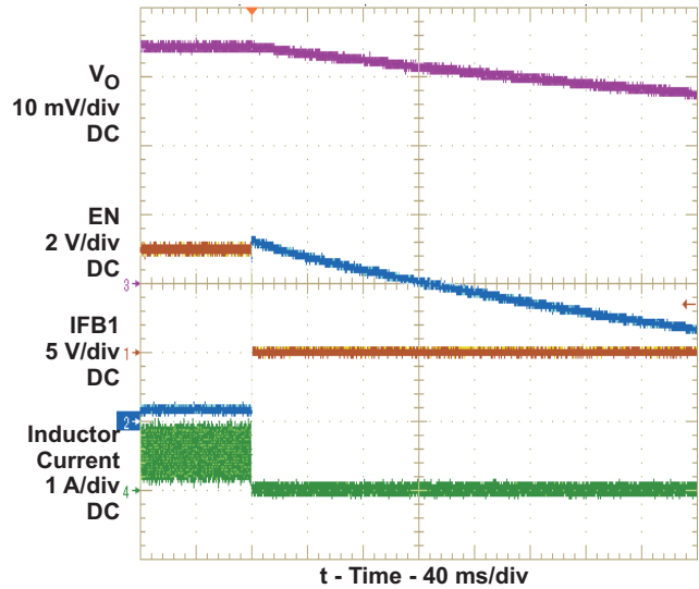
Figure 14. Shutdown Waveform
