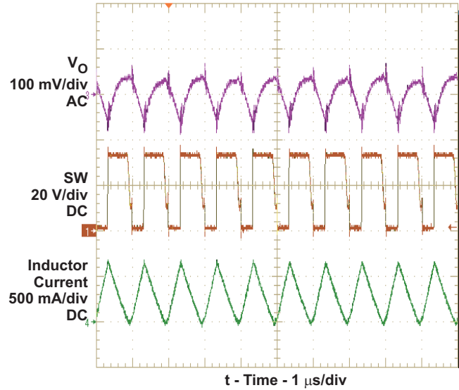
Figure 12. Switching Waveform
