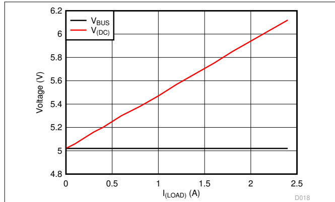
Figure 9-2. V_{(DC)} and V_{BUS} vs I_{(LOAD)} Output
