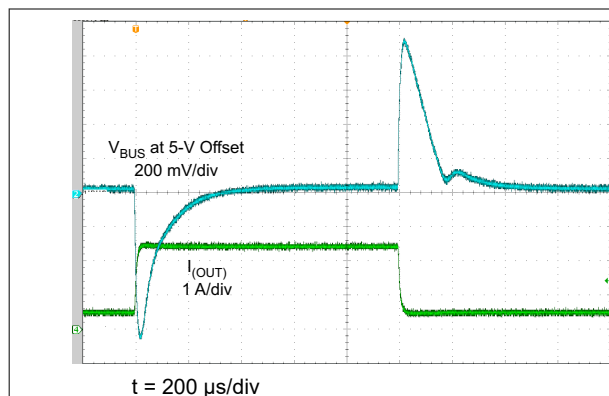
Figure 9-8. 0.5-A \leftrightarrow 2.4-A Load Transient With 100-mA/ \mu s Slew Rate, V_{BUS}
