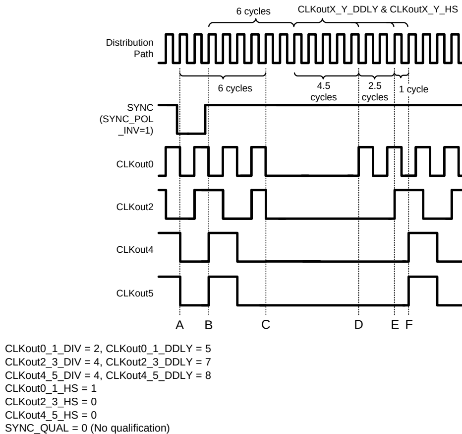
Figure 12. Clock Output Synchronization using the SYNC Pin (Active Low)
