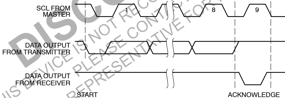
Figure 5. Acknowledge Timing
