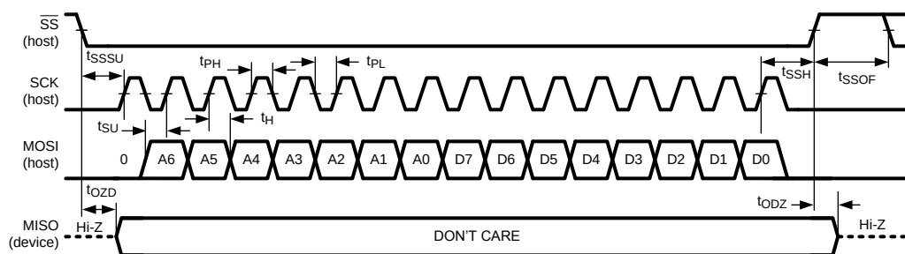
Figure 4. SPI Write
