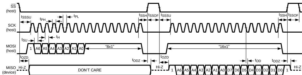
Figure 5. SPI Read
