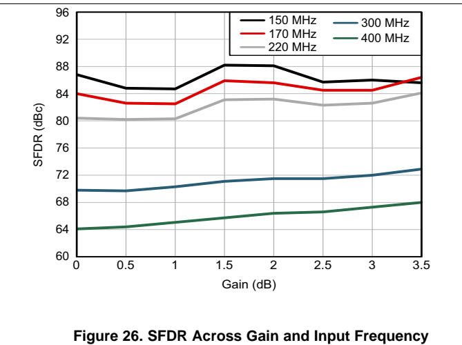
Figure 26. SFDR Across Gain and Input Frequency
