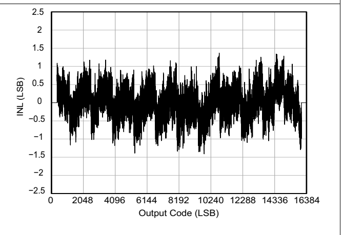
Figure 18. Integral Nonlinearity
