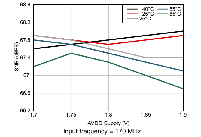
Figure 32. SNR Across Ambient Temperature vs AVDD Supply
