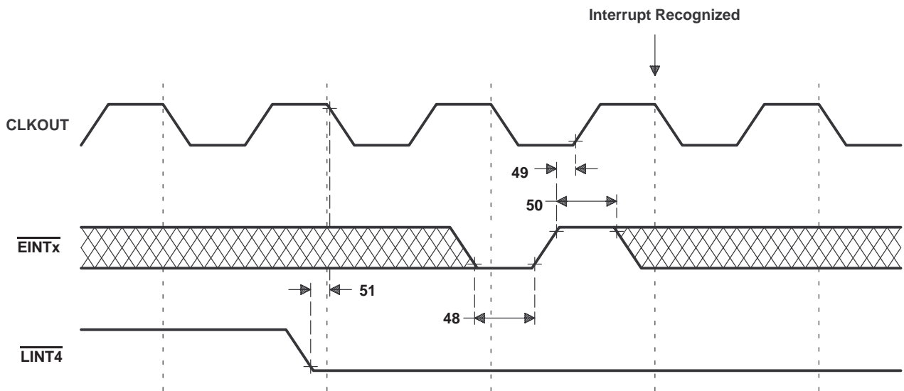
Figure 127. External-Interrupt Timing
