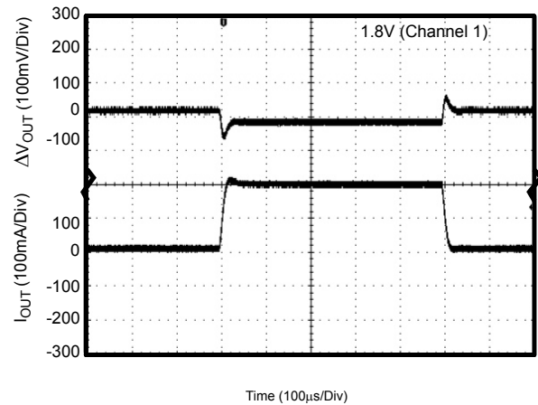
Figure 37. Load Transient
