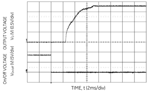
Figure 11. Typical Start-up Using Remote On/Off ( V_{IN} = V_{IN,NOM} , I_o = I_{o,max} ).
