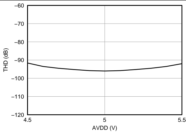
Figure 20. Total Harmonic Distortion vs Analog Supply Voltage
