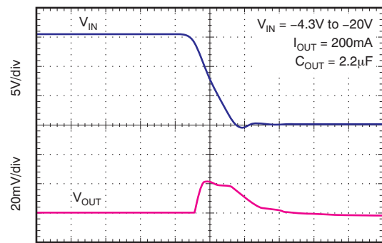
Figure 36. Line Transient Response
