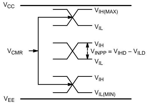
Figure 13. V_{CMR} Diagram
