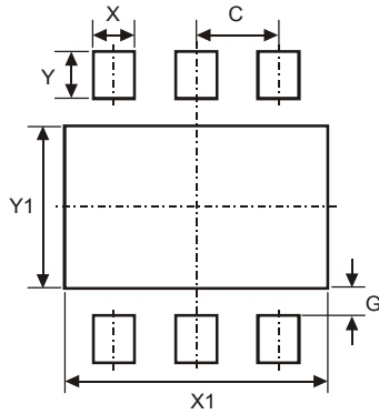
(2) U-DFN2018-6
