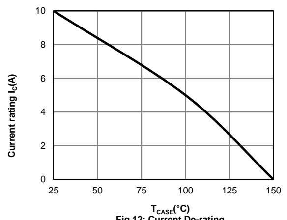
Fig 12: Current De-rating
