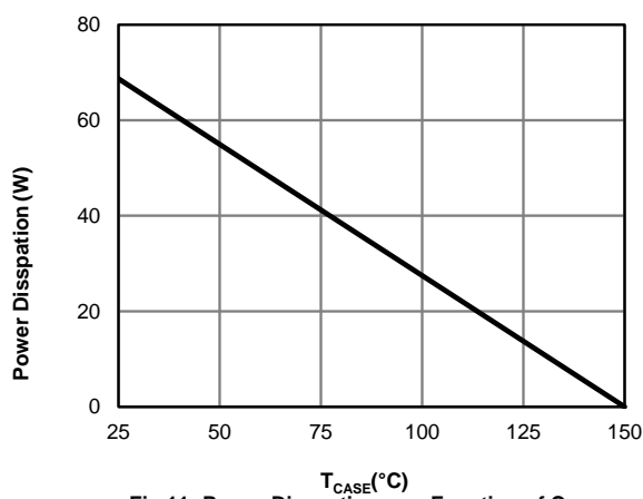
Fig 11: Power Dissipation as a Function of Case
