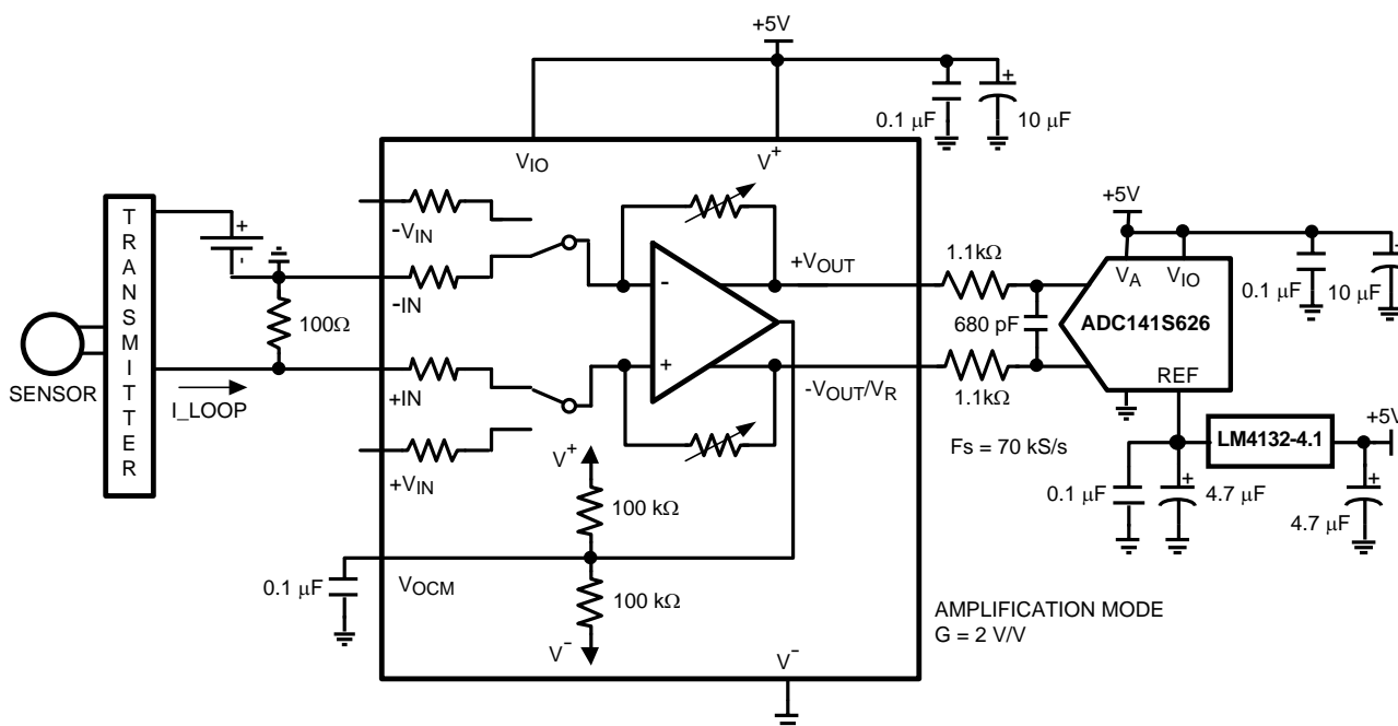
Figure 41. LMP7312 in 4-20mA Current Loop application
