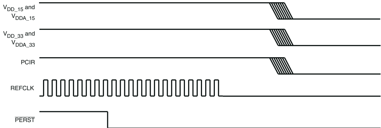
Figure 6-2. Power-Down Sequence
