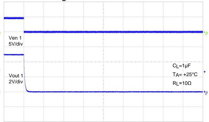
500µs/div Channel 1 Turn-Off Delay and Fall Time
