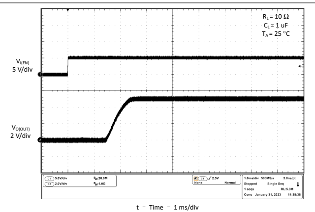
Figure 7-40. Turnon Delay and Rise Time With 1- \mu F Load
