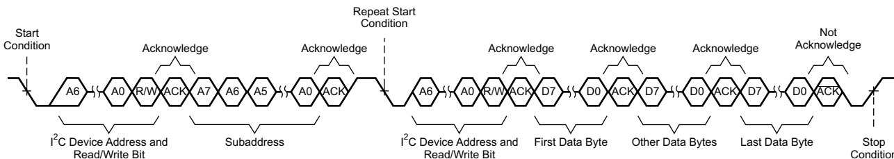
Figure 20. Sequential Read Transfer
