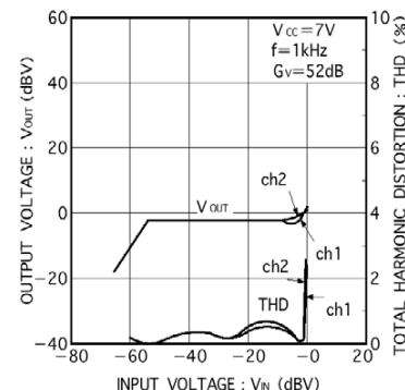
Fig.10 ALC characteristics
