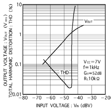
Fig.11 Input/output characteristics
