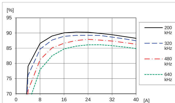
Efficiency vs. Output Current and Switching Frequency
