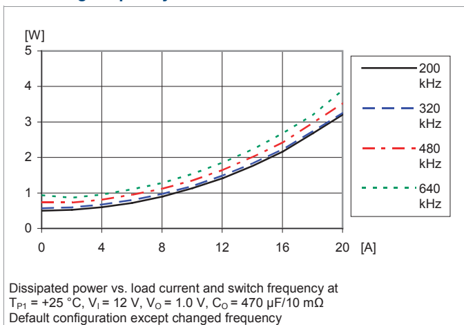
Power Dissipation vs. Output Current and Switching frequency
