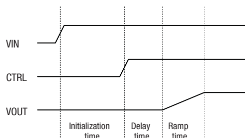
Illustration of Power Up Procedure
