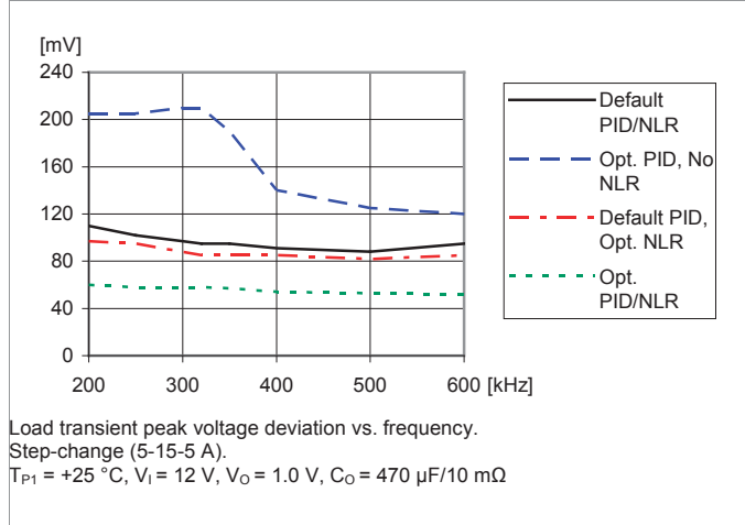
Load transient vs. Switch Frequency
