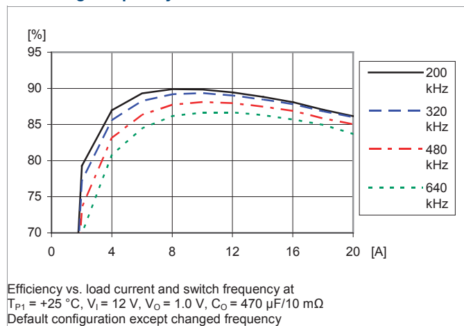
Efficiency vs. Output Current and Switching Frequency
