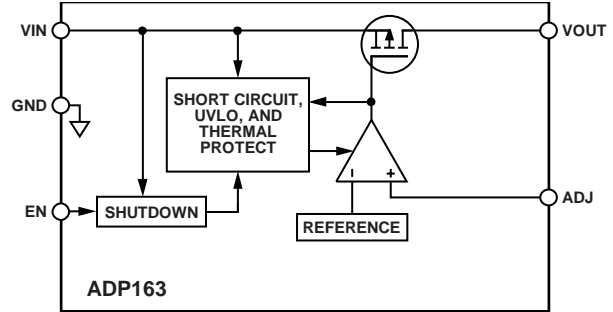
Figure 33. Internal Block Diagram, Adjustable Output without Output Discharge Function
