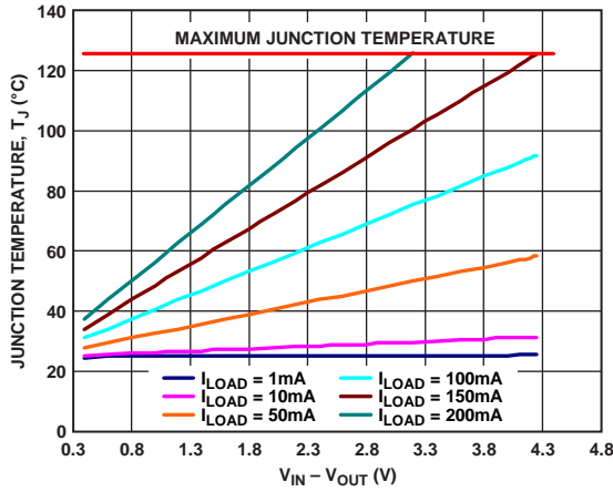
Figure 42. 100 mm 2 of PCB Copper, WLCSP, T_A = 50^\circ\text{C}
