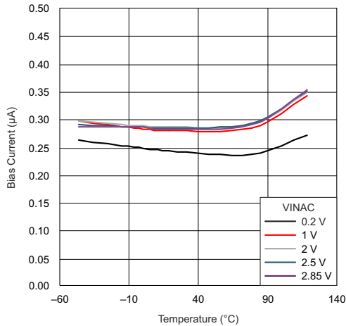
Figure 5-7. I_{VINAC} Bias Current vs Junction Temperature
