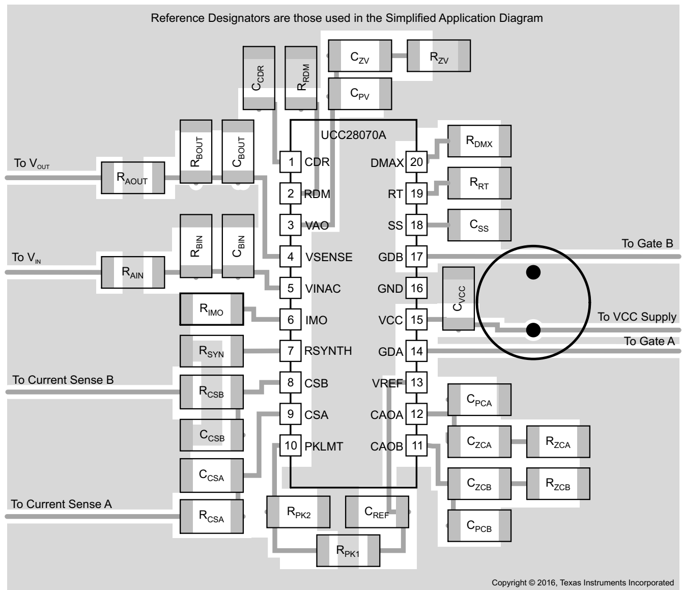
Figure 7-10. Layout Diagram
