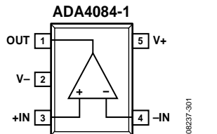
Figure 4. ADA4084-1, 5-Lead SOT-23 (RJ)
