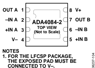
Figure 5. ADA4084-2, 8-Lead LFCSP (CP)
