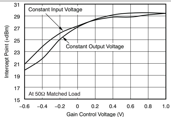
Figure 64. Two-Tone, Third-Order Intermodulation Intercept vs Gain Control Voltage ( f_{IN} = 20\text{ MHz} )
