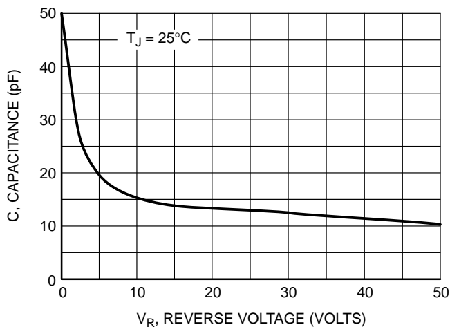
Figure 7. Maximum Capacitance
