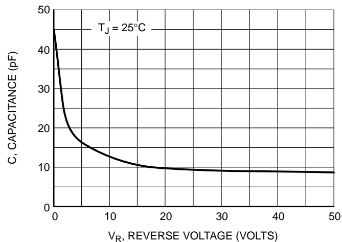
Figure 8. Typical Capacitance
