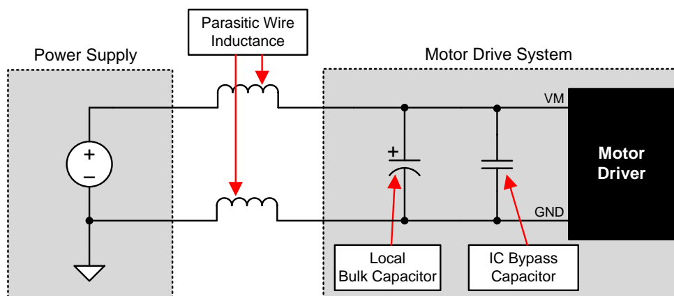
Figure 41. Example Setup of Motor Drive System With External Power Supply
