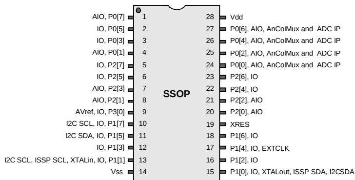
Figure 4. CY8C24633 PSoC Device
