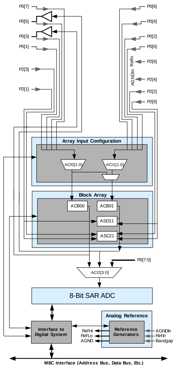
Figure 3. Analog System Block Diagram
