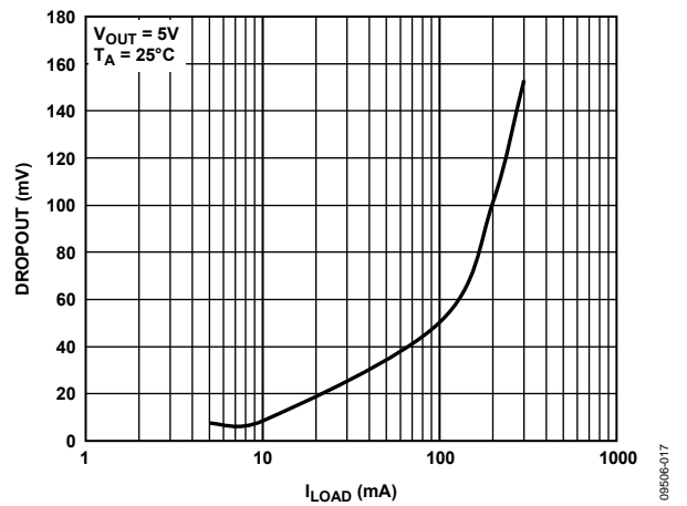
Figure 21. Dropout Voltage vs. Load Current, V_{OUT} = 5 V
