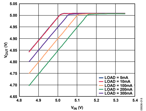
Figure 22. Output Voltage vs. Input Voltage (in Dropout), V_{OUT} = 5 V
