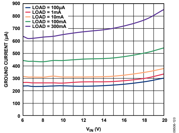
Figure 20. Ground Current vs. Input Voltage, V_{OUT} = 5 V
