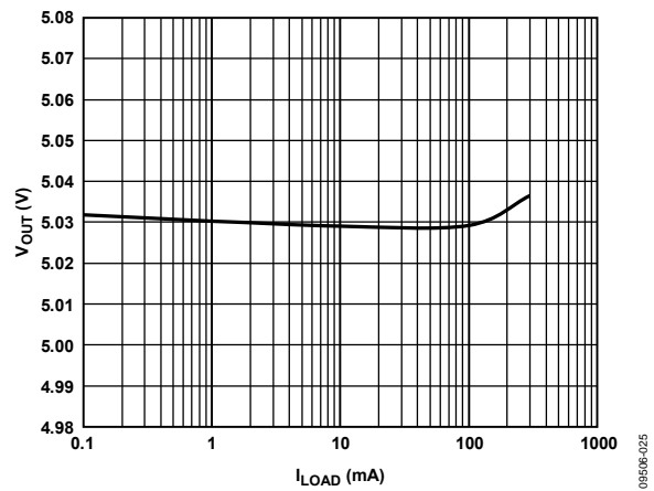
Figure 31. Output Voltage vs. Load Current, V_{OUT} = 5 V , Adjustable
