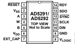
Figure 5. Pin Configuration
