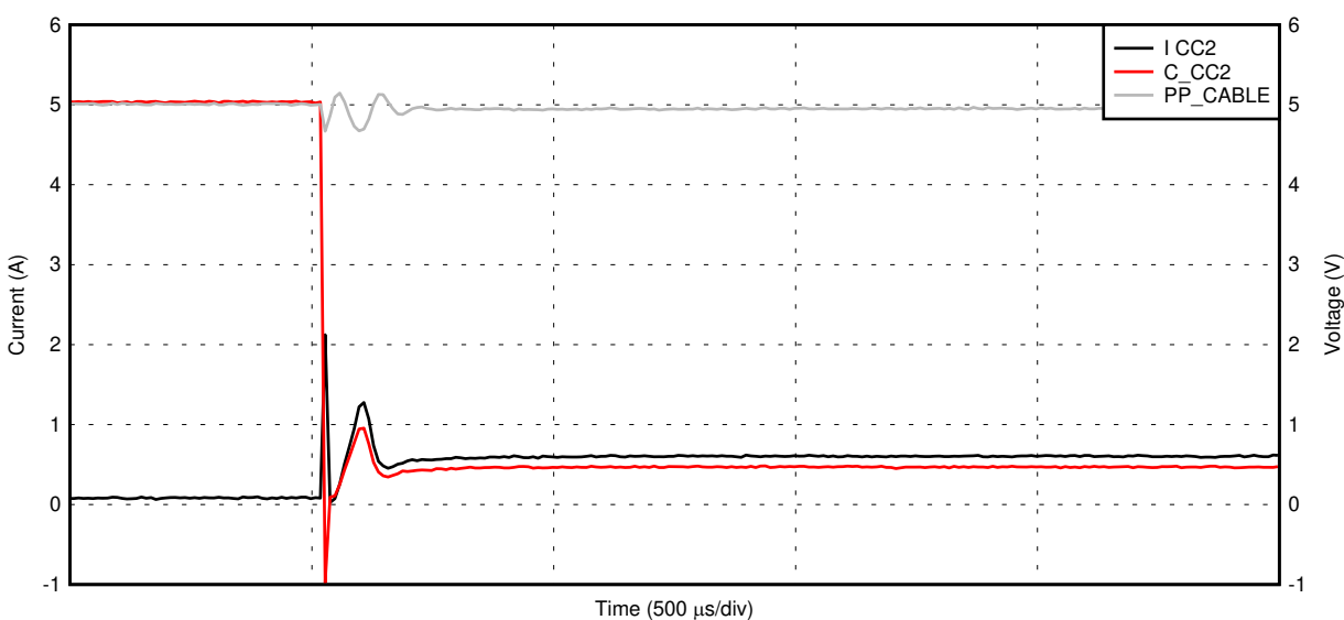
Figure 9-32. PP_CABLE to C_CCn Current Limit with a Hard Short (Extended Time Base)
