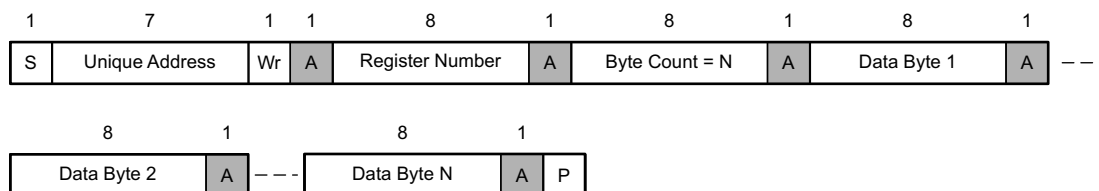
Figure 9-64. I²C Unique Address Write Register Protocol
