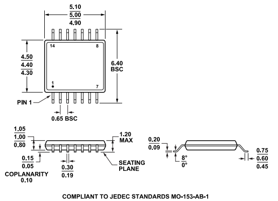
Figure 93. 14-Lead Thin Shrink Small Outline Package [TSSOP] (RU-14) Dimensions shown in millimeters
