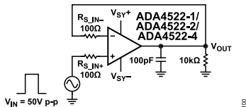
Figure 75. Circuit Diagram for Large Signal Transient Response
