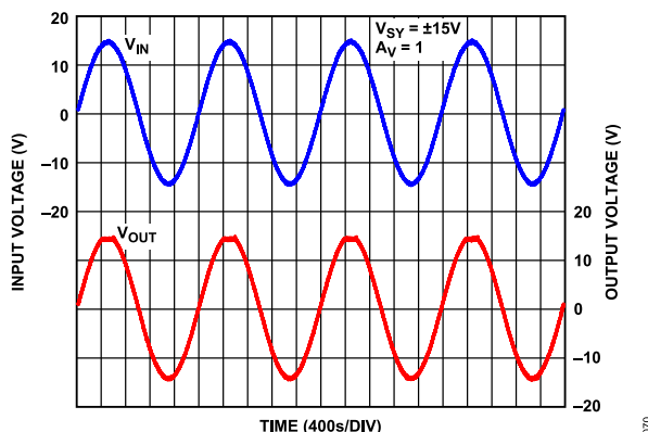
Figure 73. Input and Output Waveforms, No Phase Reversal
