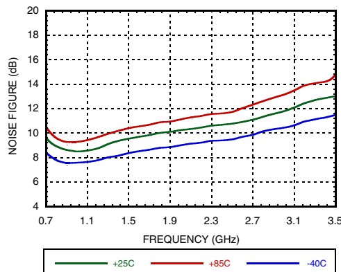
Figure 21. Noise Figure vs. Temperature @ VGATE=5.0V
