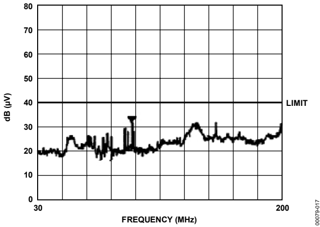
Figure 22. Radiated Emissions
