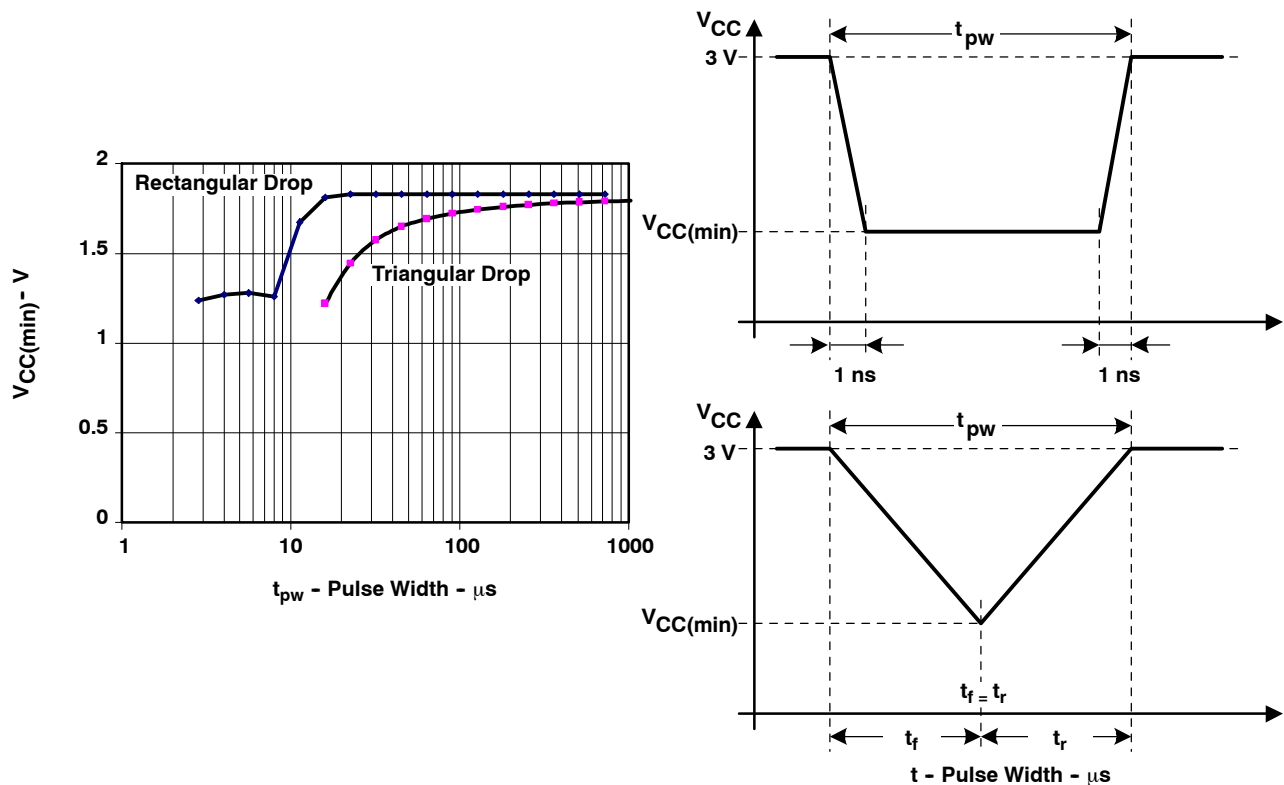
Figure 12. V_{CC(min)} With a Square Voltage Drop and a Triangle Voltage Drop to Generate an SSVS Signal
