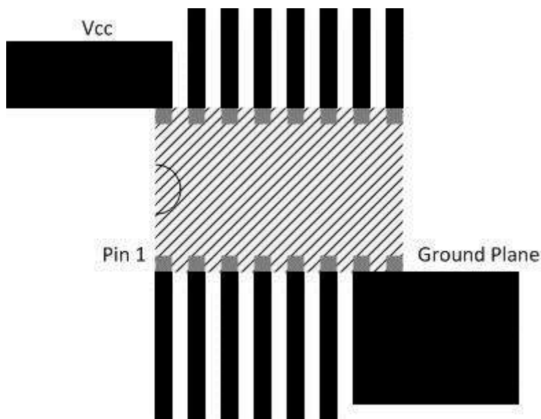
Figure 8-2. Layout Schematic
