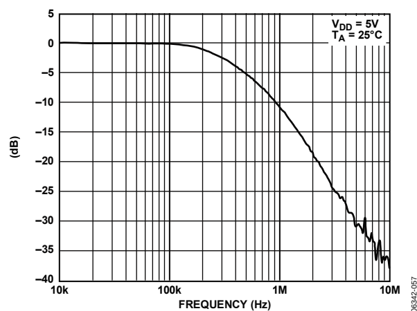
Figure 51. Multiplying Bandwidth
