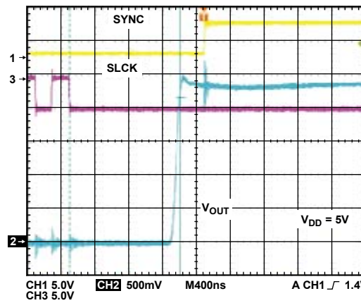
Figure 41. Exiting Power-Down to Midscale
