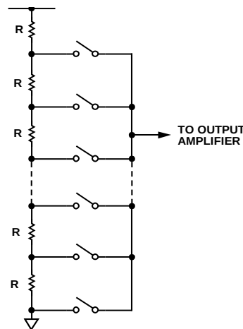
Figure 53. Resistor String
