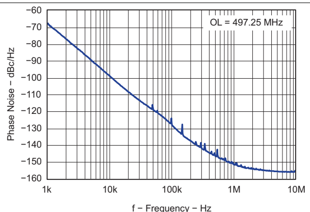
Figure 61. Open Loop VCO Phase Noise
