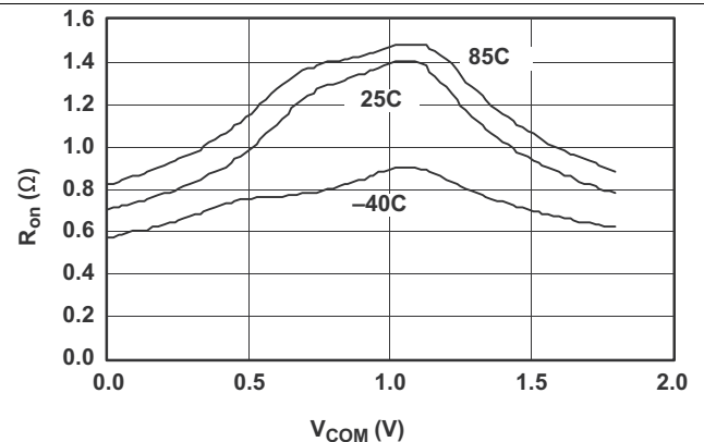
Figure 2. R_{on} vs V_{COM} ( V_{CC} = 1.8 V)
