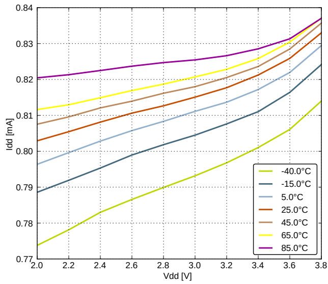
Figure 4.5. EM0 Current Consumption while Executing Prime Number Calculation Code from Flash with HFRCO Running at 6.6 MHz
