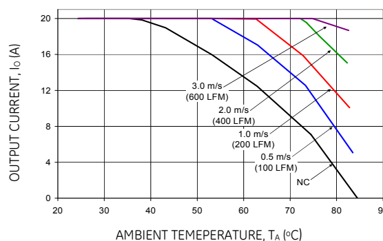
Figure 16. Output Current Derating for the Module with Heatplate; Airflow in the Transverse Direction from Vout(+) to Vout(-); Vin = 48V.
