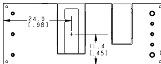
Figure 20. Pick and Place Location.
