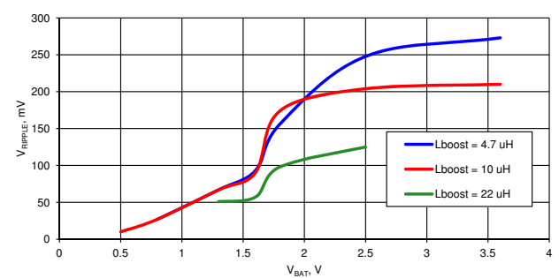
Figure 11-14. V_{RIPPLE} vs V_{BAT} [34]
