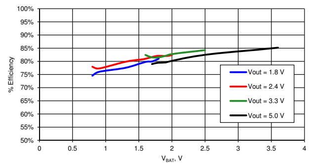
Figure 11-12. Efficiency vs V_{BAT} , L_{BOOST} = 10 \mu H [34]
