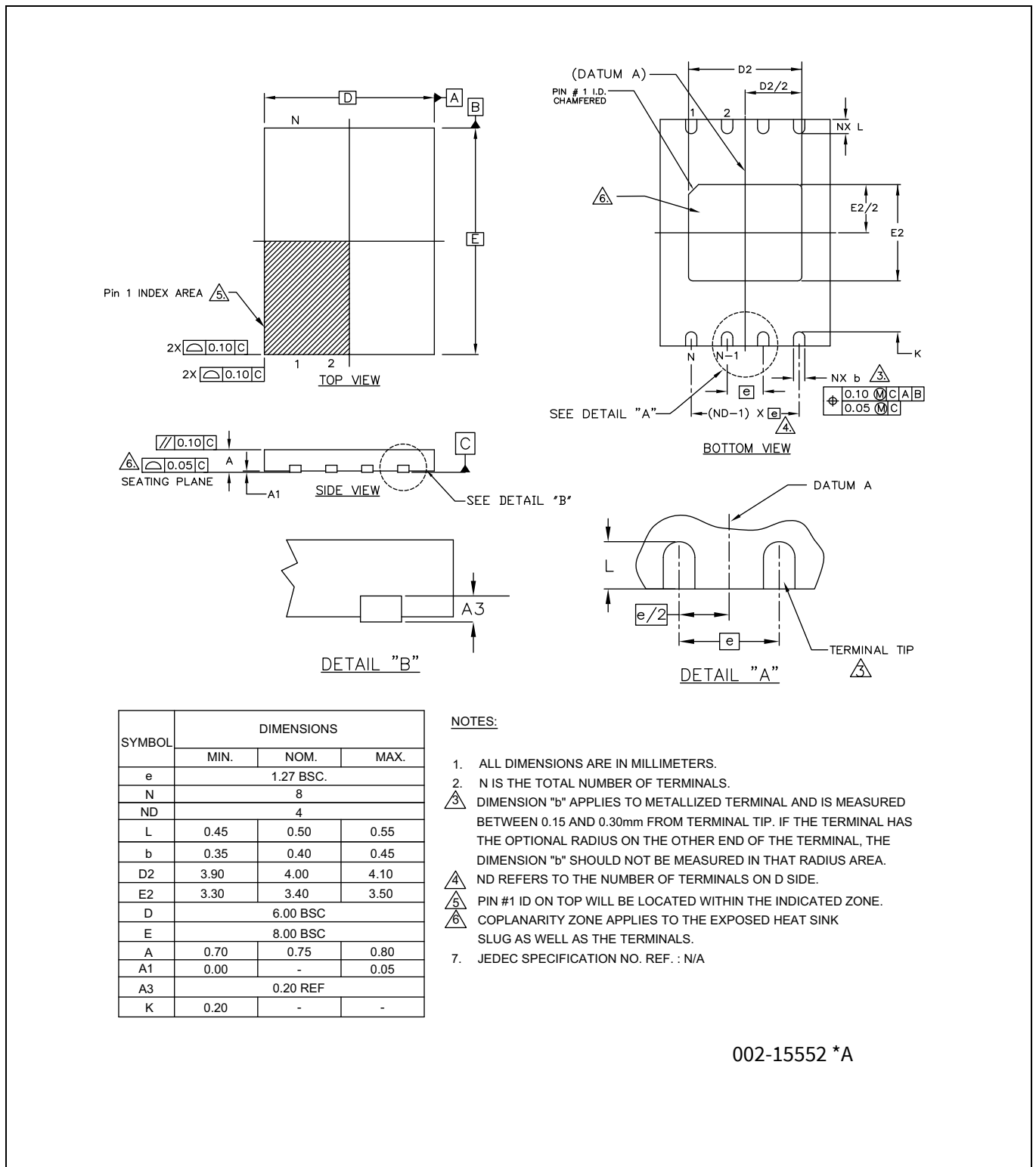
Figure 42 8-lead DFN ((6.0 × 8.0 × 0.8 mm) 4.0 × 3.4 mm E-pad (sawn)) package outline, 002-15552
