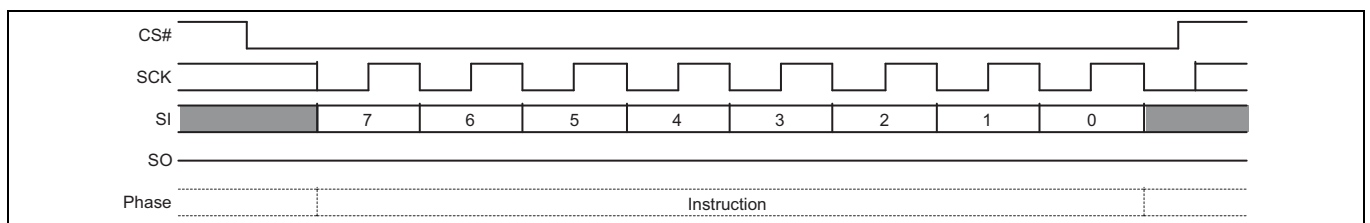
Figure 93 Bulk Erase command sequence
