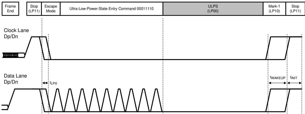
Figure 31. Ultra-Low-Power State
