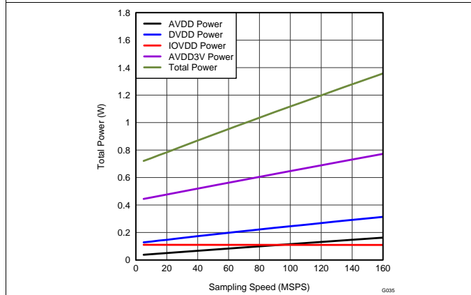
Figure 40. Total Power vs Sampling Frequency
