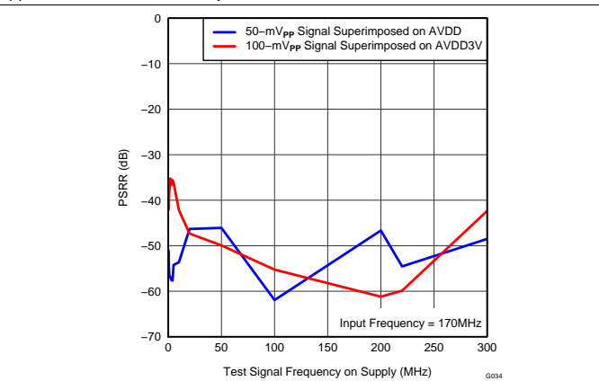
Figure 39. Power-Supply Rejection Ratio vs Test Signal Frequency
