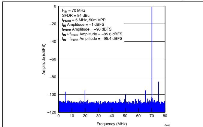
Figure 38. Power-Supply Rejection Ratio FFT for AVDD Supply
